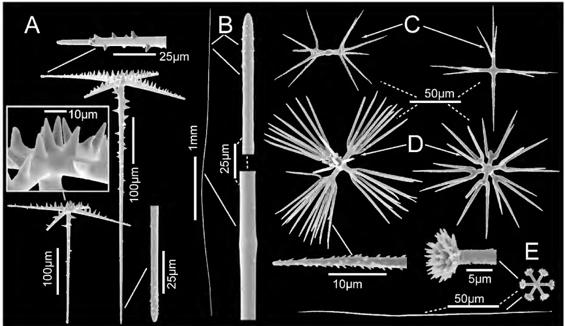
FIG. 4. Atlantisella lorraineae sp. nov., holotype NIWA 82163, spicules. A, two surficial pentactins, whole and enlarged ray ends and center; B, diactin, whole and enlarged end and middle segments; C, oxystaurasters in side and facial views; D, calycocome-like oxyhexasters with differing terminal ray numbers and an enlarged terminal ray end; E, graphiocomes centrum and loose terminal ray.
